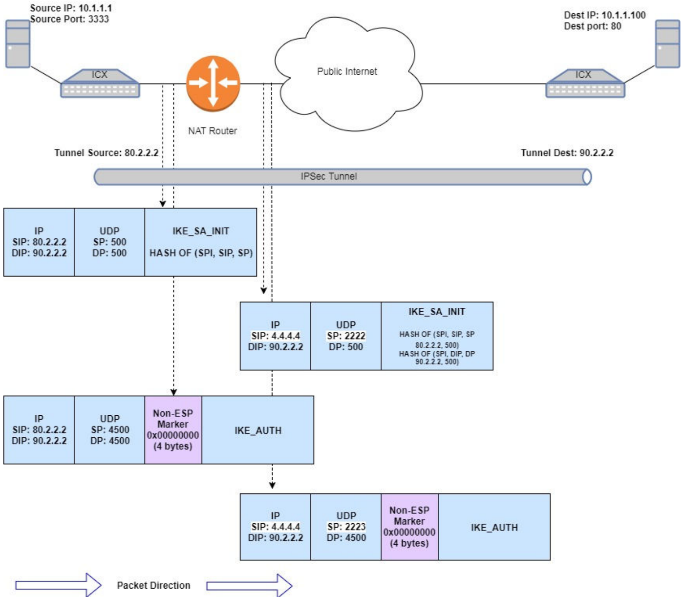
FIGURE 24 IPsec over NAT- Control flow
