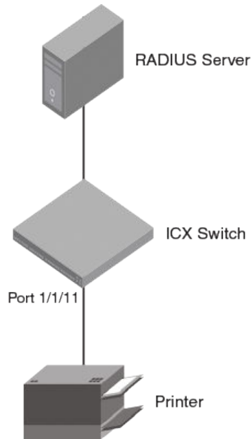
FIGURE 21 802.1X authentication and MAC authentication enabled on the same port
