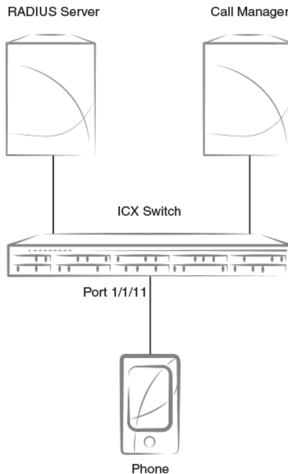
FIGURE 18 Authenticating an IP phone when RADIUS does not return a VLAN assignment
