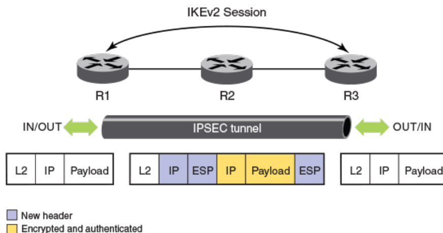
FIGURE 23 Basic IPsec functionality
